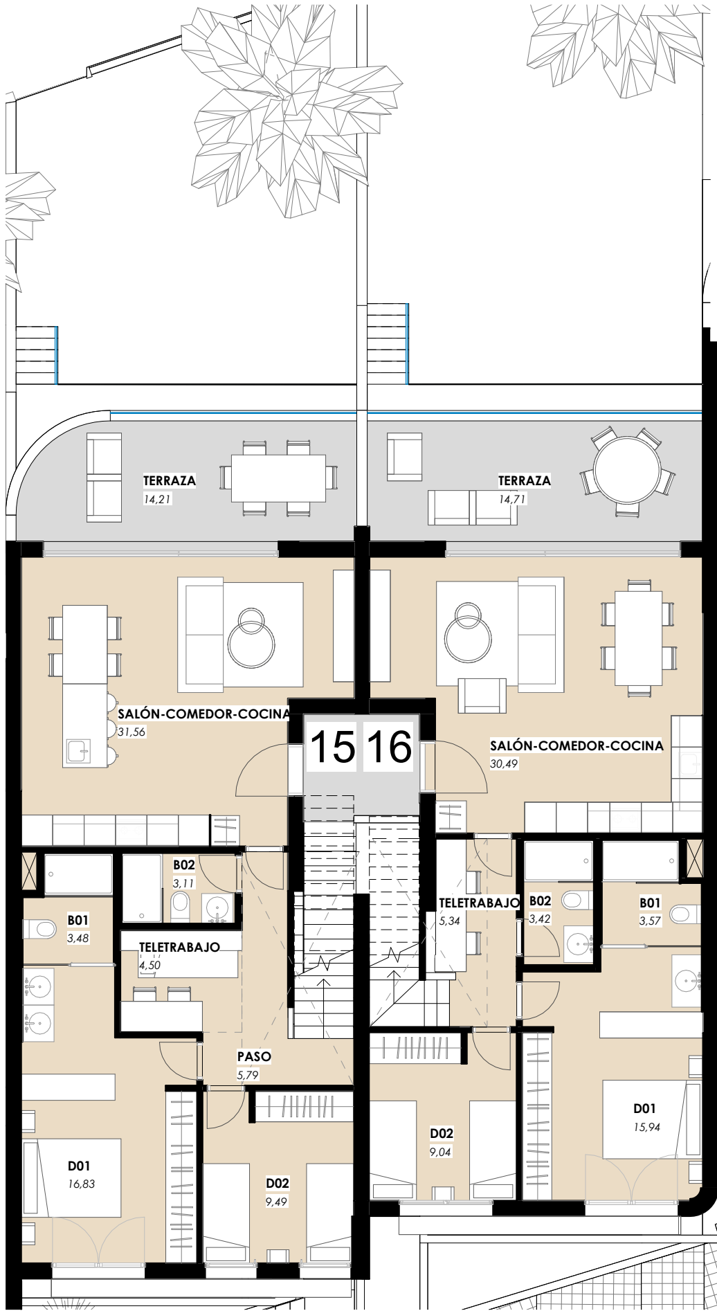
VIVIENDA 15-16_PLANTA PRIMERA/ APARTMENT 15-16_TOP FLOOR 1 : 100
